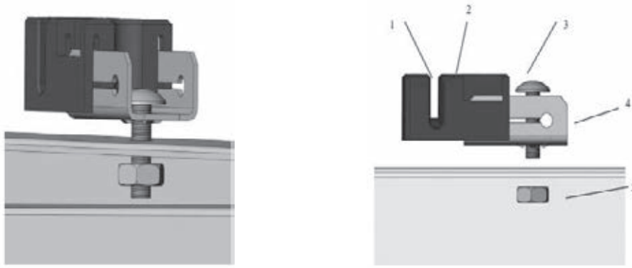
Fig: Grounding bolt # 1954381-2
