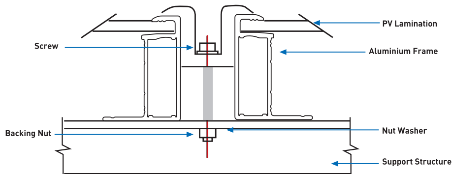
Fig 5 PV modules installed using fringe clamping method
